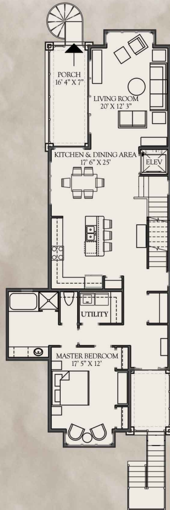
FIRST FLOOR 1,400 SQ. FT. HEATED 201 SQ. FT. PORCHES
