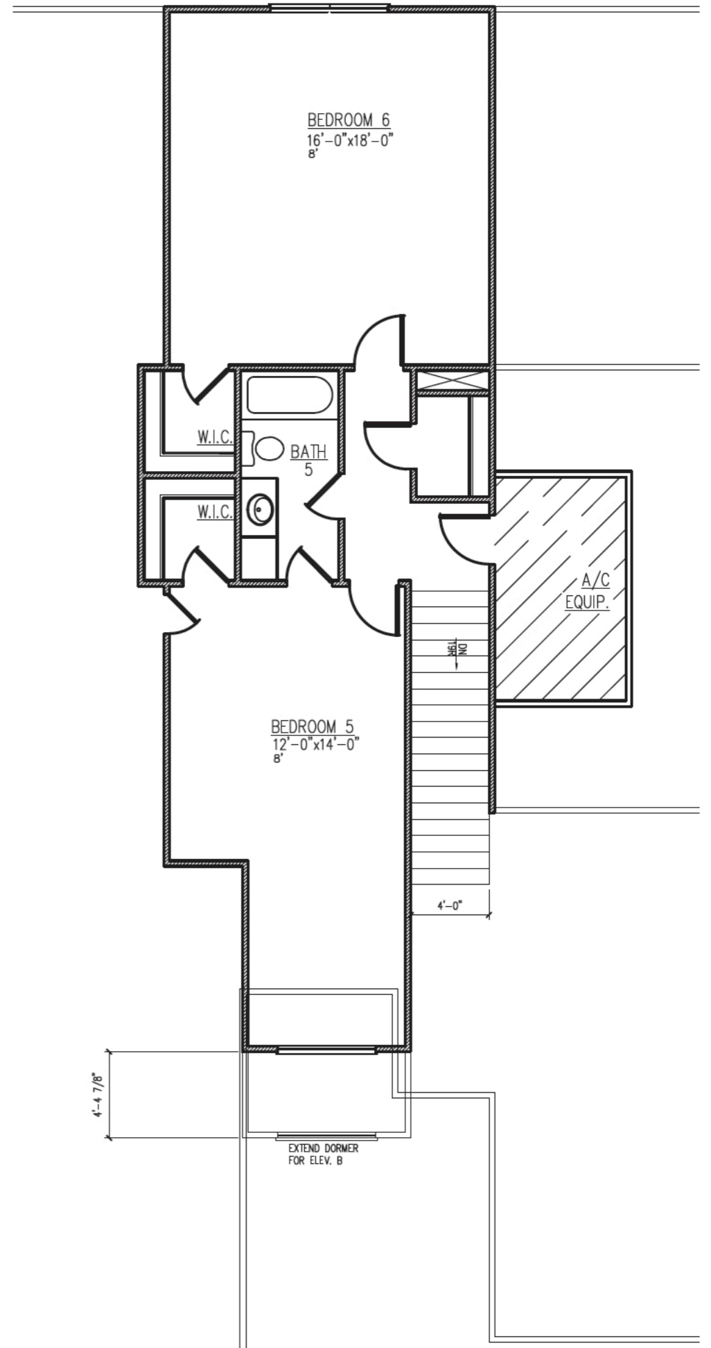
Second Floor
