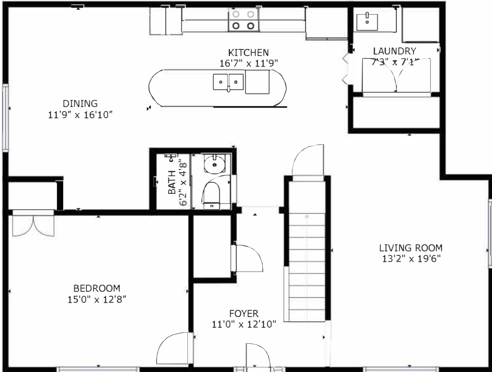
FLOOR 1
