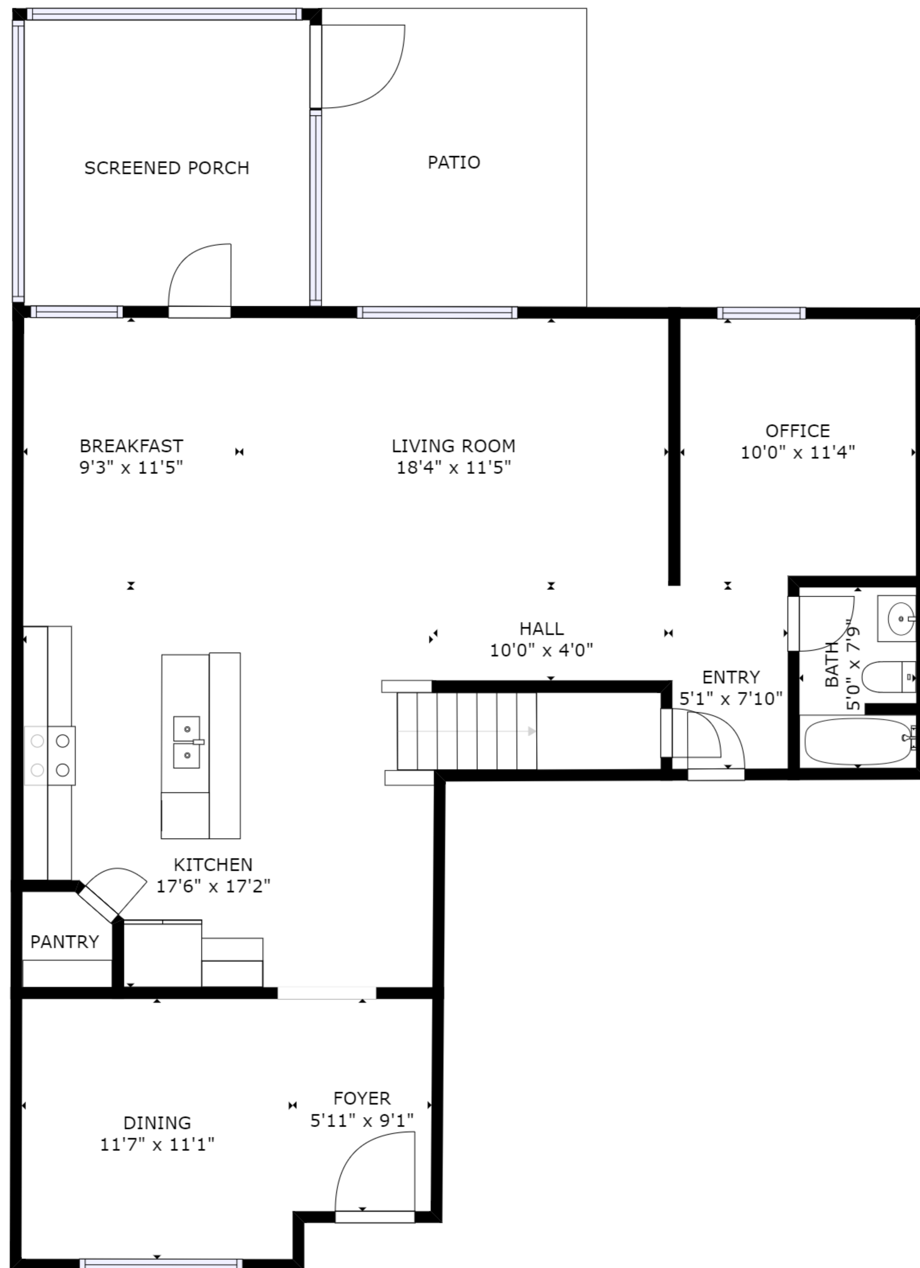
FLOOR 1
