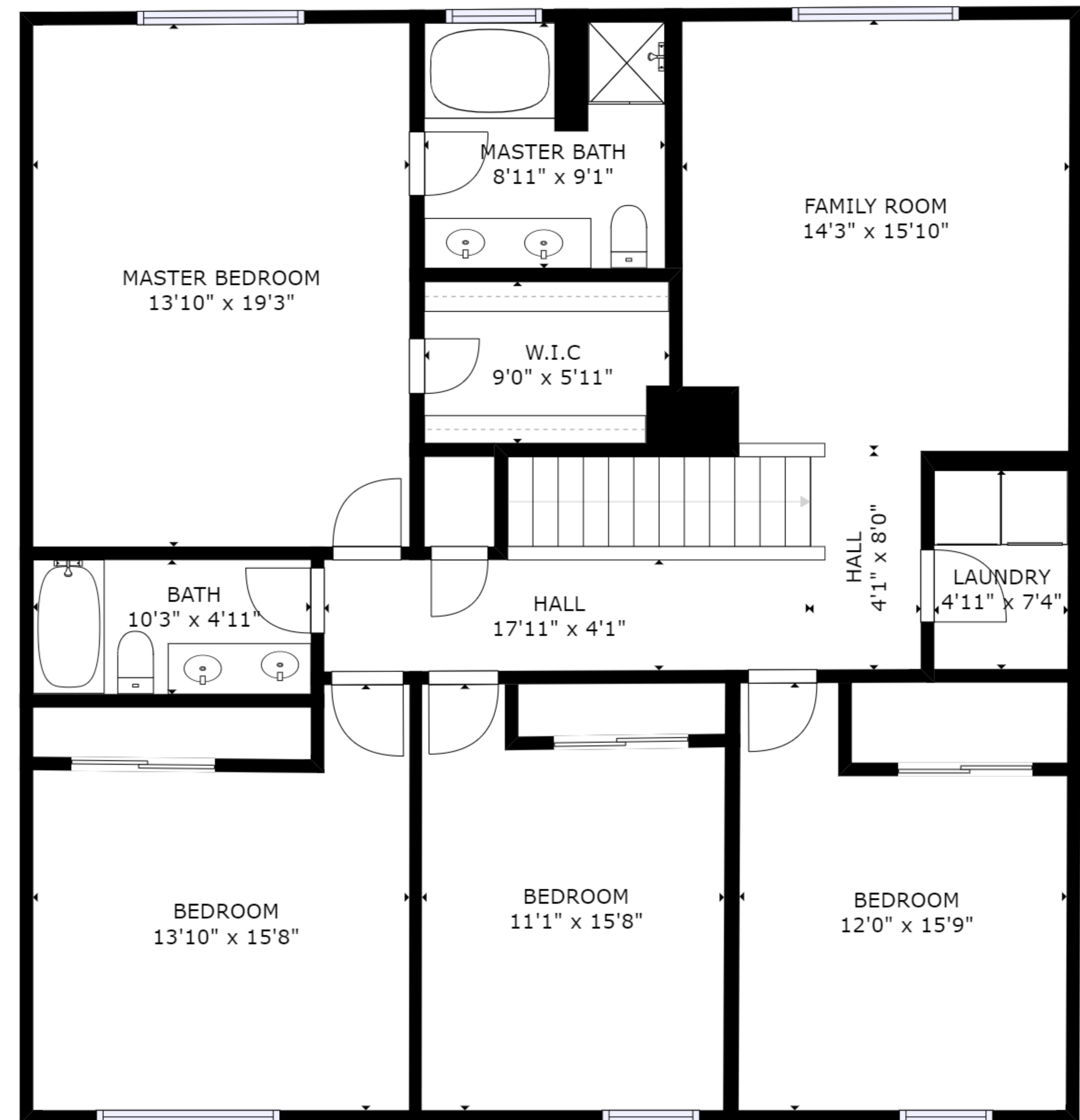
FLOOR 2
