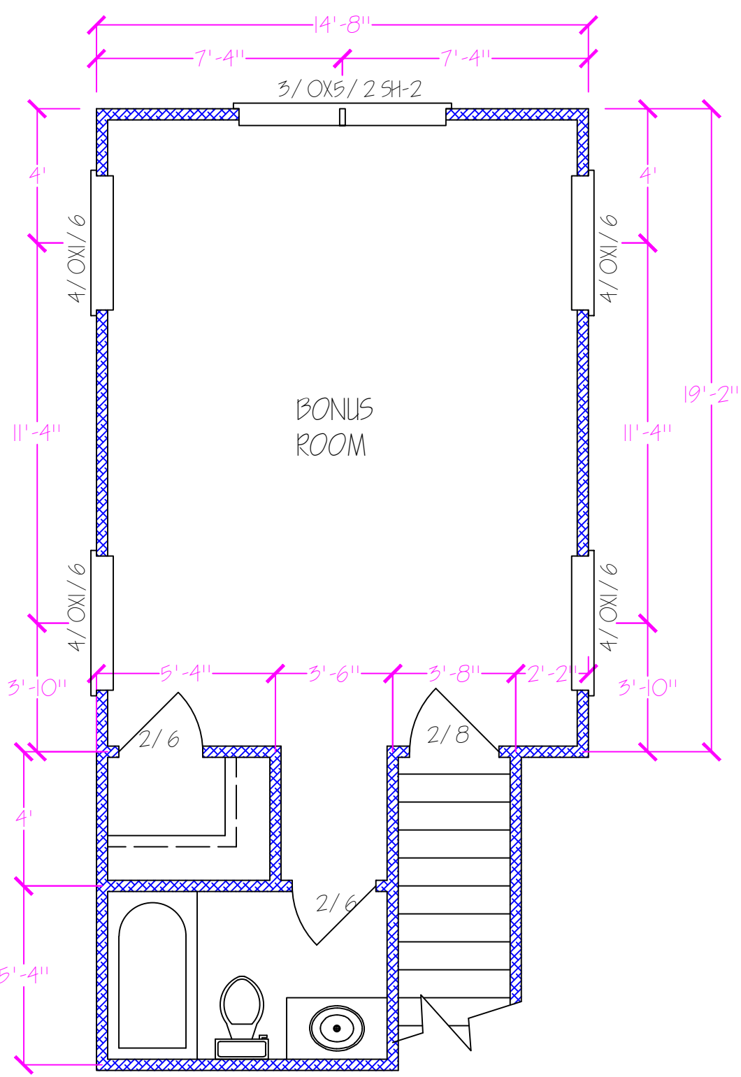
BONUS PLAN 368 SQ.FT. HEATED 1/ 4 INCH SCALE
