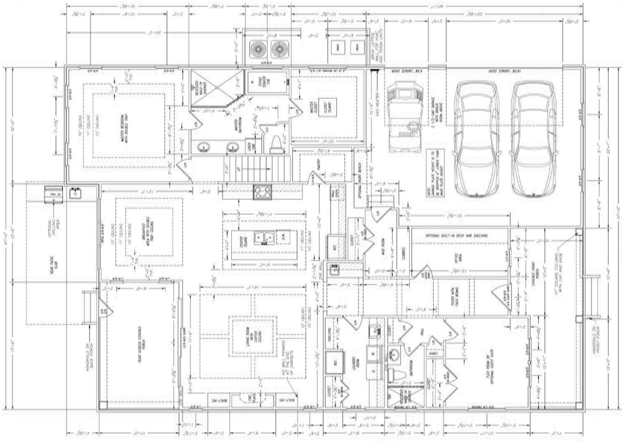
FIRST FLOOR SCALE: 1/4" = 1'-0"
