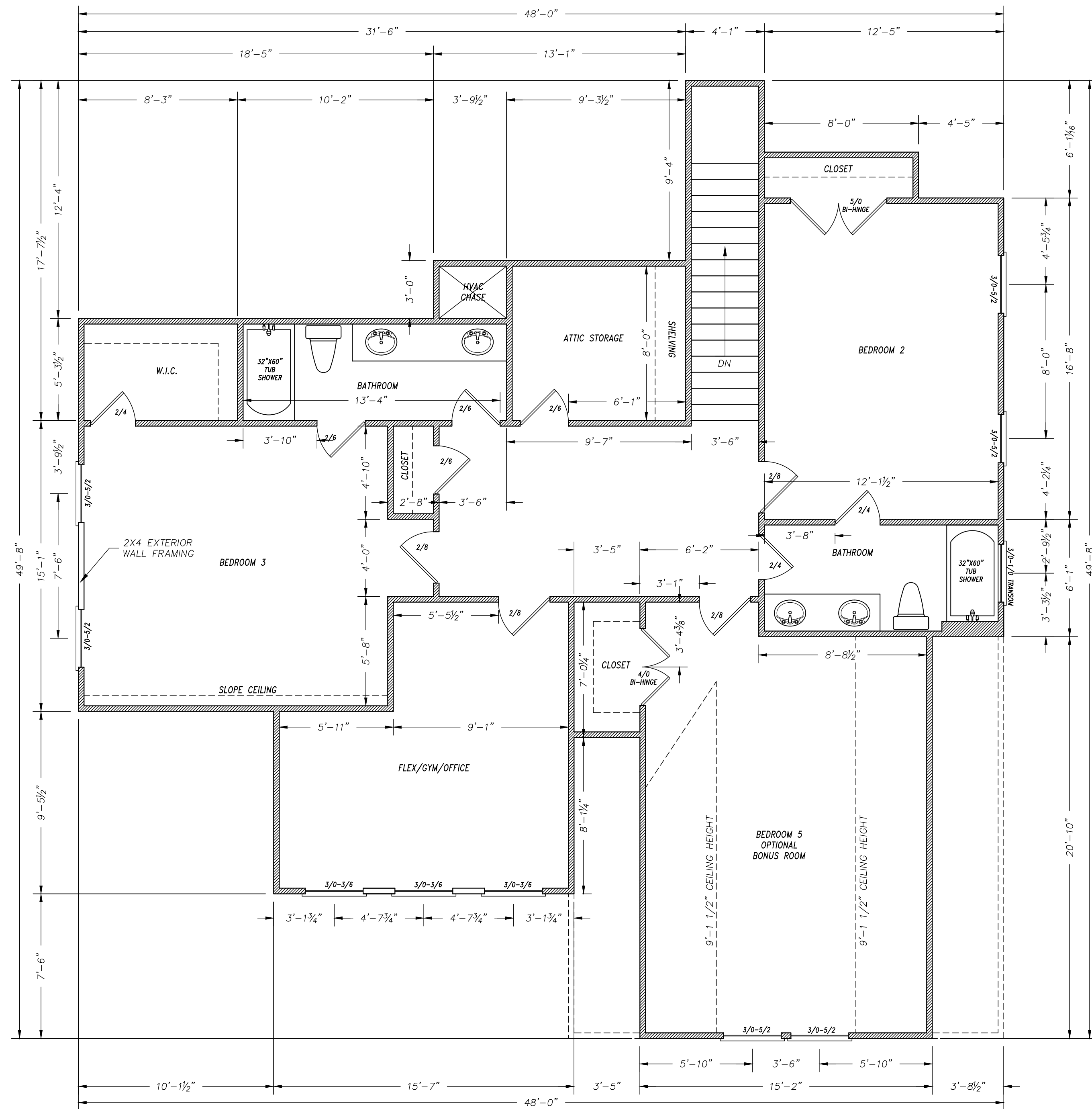
SECOND FLOOR SCALE: 1/4" = 1 FT.
