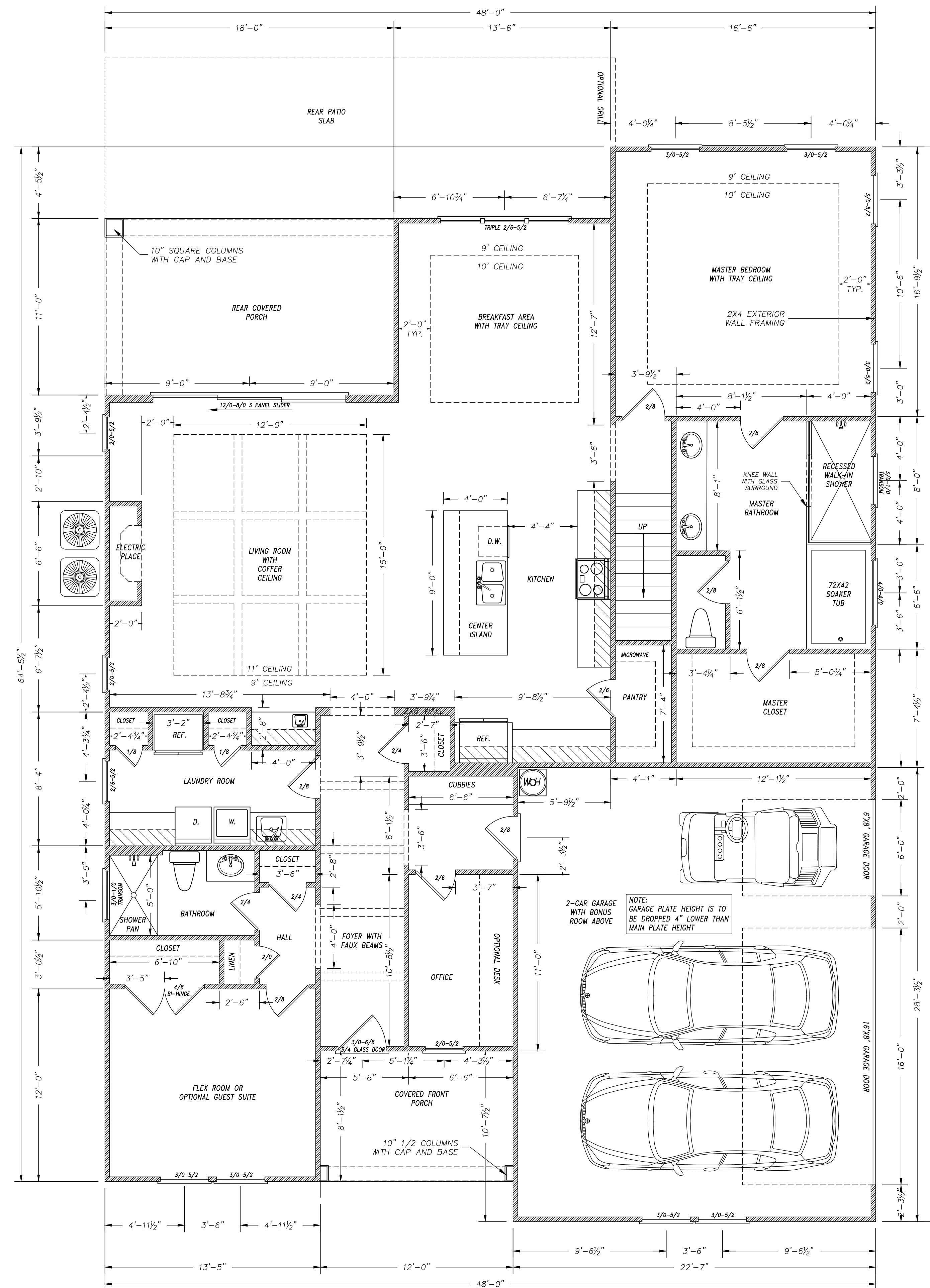
FIRST FLOOR SCALE: 1/4" = 1 FT.
